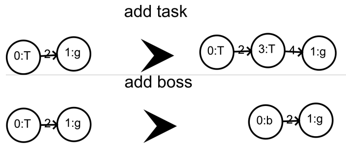
Fig. 5.11: Two new rules to replace the old "add task"
